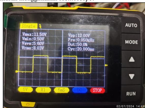
Gambar 12. Output 1LO IR2110
