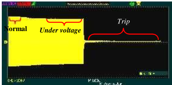
Gambar 4.3 Gelombang Tegangan Under Voltage 285 V
