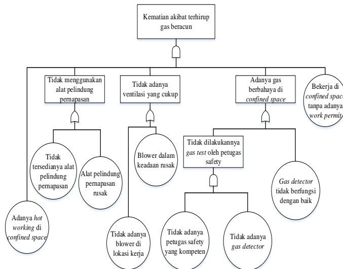
Gambar 1. Diagram FTA Kematian Akibat Terhirup Gas Beracun
