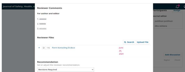
Gambar 20. Komen Reviewer
