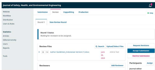
Gambar 8. Upload File
