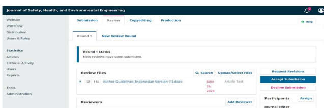
Gambar 21. Request Revision
