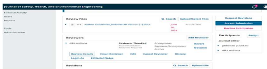
Gambar 19. Review Detail
