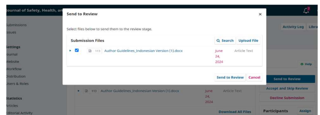
Gambar 7. Submission Requirements
