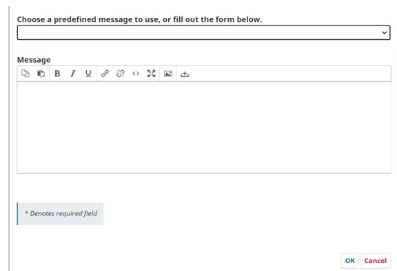
Gambar 4. Klik Ok
