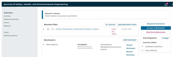
Gambar 18. Thank Reviewer
