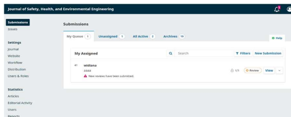
Gambar 15. View
