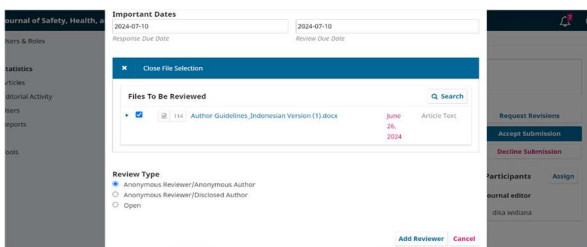
Gambar 10. Article Text
